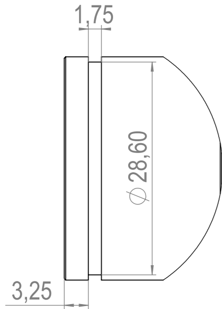
A (2:1)
